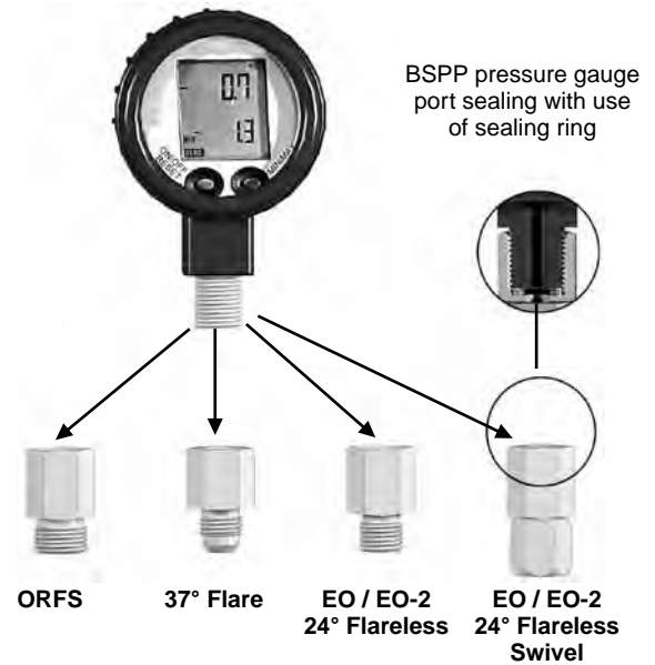
Fig. M4 — BSPP pressure gauge connections
